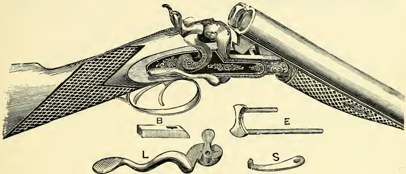
Side-lever Breech-loader with Bar, or Front-action, Locks.
